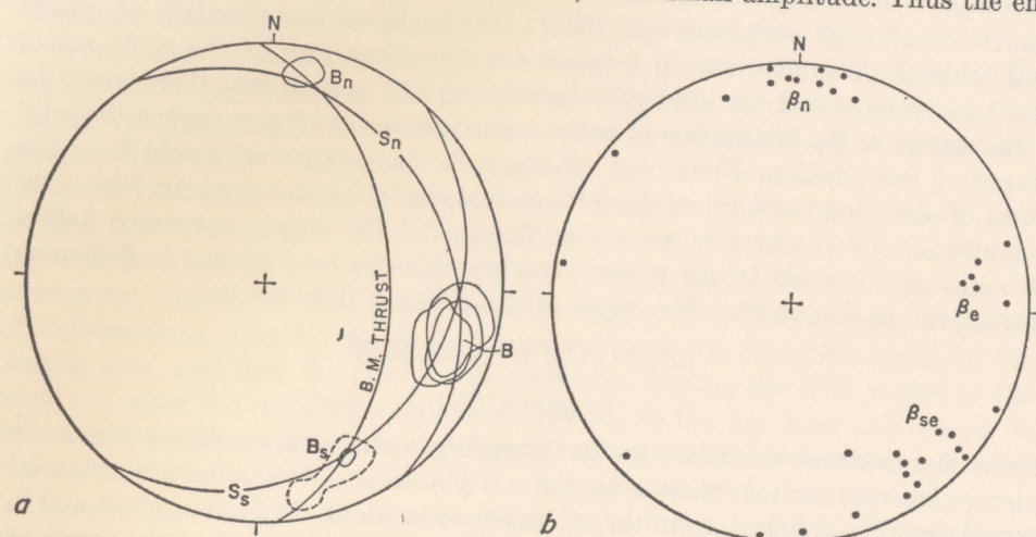
Fig. 24. a . Synoptic diagram showing maxima of fold axes in Stack of Glencoul area ( B , B_n ), Loch Ailsh area ( B ), and Cnoc a' Chaoruinn area ( B , B_n ). S_n and S_s represent the mean orientations of the foliation in the northern and southern areas, respectively. The mean orientation of the Ben More thrust is also shown. Full lines are 10 per cent contours, and the broken line is a 6 per cent contour. b . Synoptic diagram showing the orientation of \beta -axes in Cambrian and Torridonian rocks in zone of dislocation (from fig. 20, in pocket).
